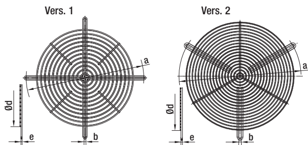
Air intake guard grilles for backward curved centrifugal fans (according to EN ISO 13857)
