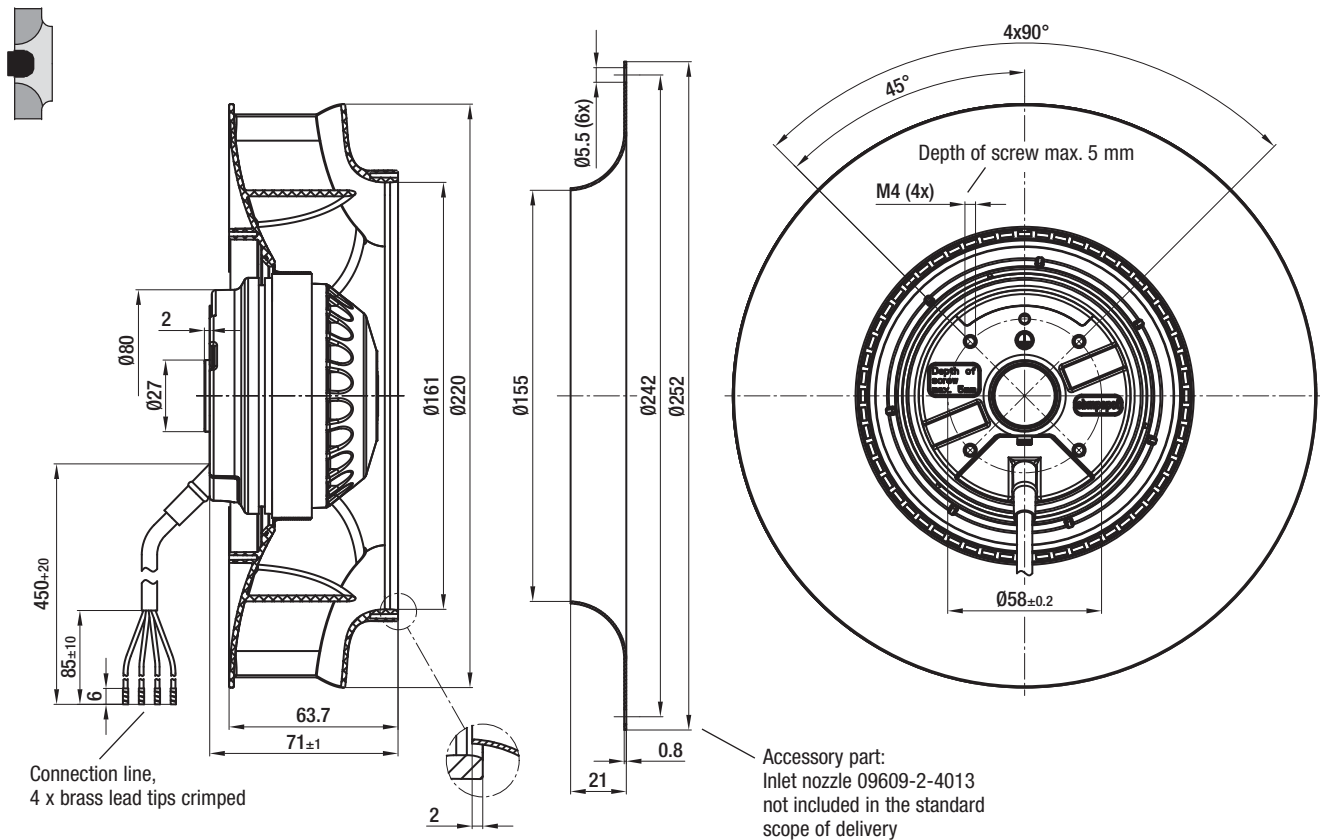
K2E 220-RA38-01 / K2E 220-RB06-01 (Centrifugal module with support basket)
