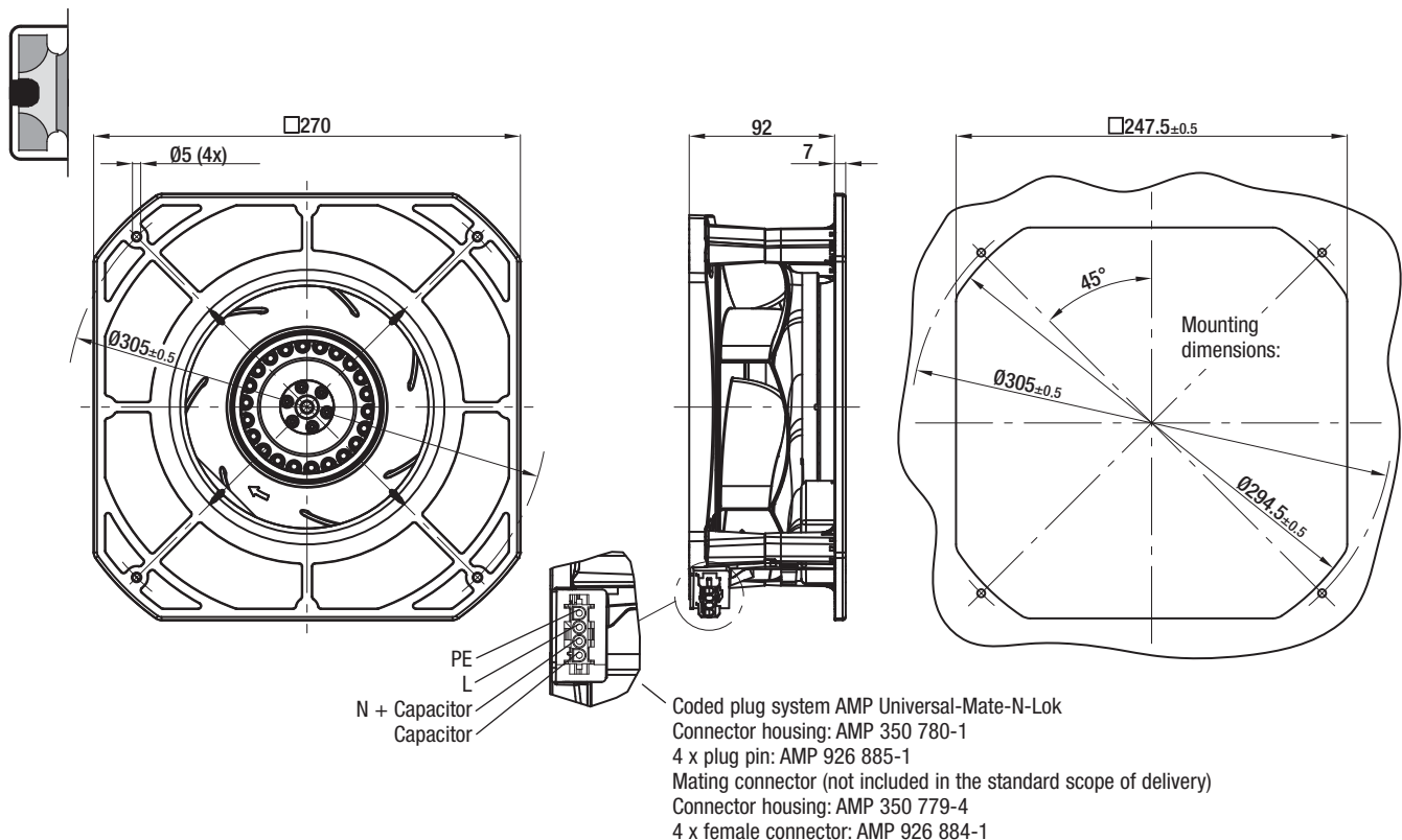
K2E 220-RA38-01 / K2E 220-RB06-01 (Centrifugal module with support basket)
